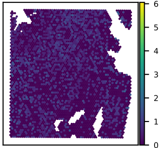
SNU51A RCSD1 expression Moran's I = 0.05
