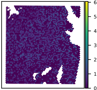
SNU51A LFNG expression Moran's I = 0.03
