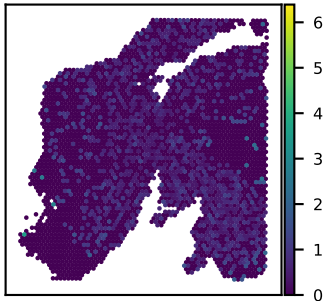
SNU24A IGF2BP2 expression Moran's I = 0.06
