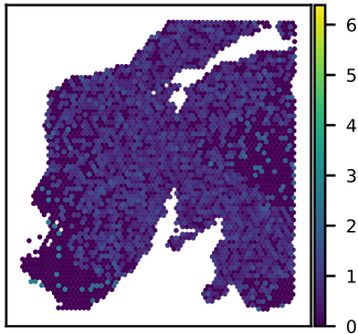
SNU24A HNRNPF expression Moran's I = 0.06
