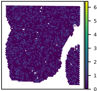
SNU25B SLC10A7 expression Moran's I = 0.01
