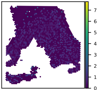
SNU18A CASTOR1 expression Moran's I = 0.05
