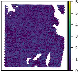
SNU51A QSOX1 expression Moran's I = 0.04
