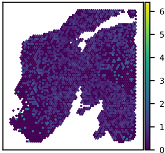
SNU24A TTC13 expression Moran's I = 0.03
