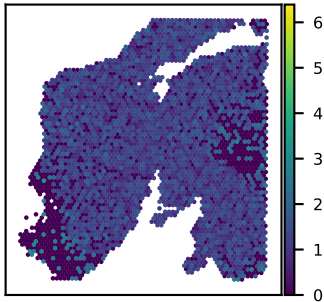
SNU24A FAM50A expression Moran's I = 0.10
