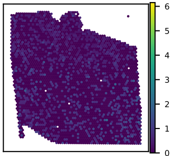
SNU27A CDK20 expression Moran's I = 0.02
