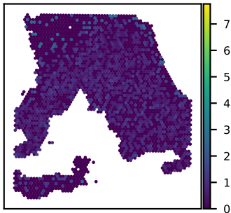
SNU18A BLVRB expression Moran's I = 0.03
