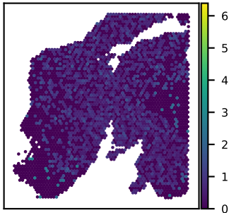
SNU24A UHRF1BP1 expression Moran's I = 0.07
