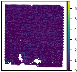
SNU43A PACRGL expression Moran's I = 0.02
