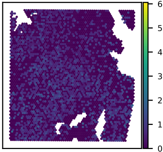
SNU51A NDC80 expression Moran's I = 0.08
