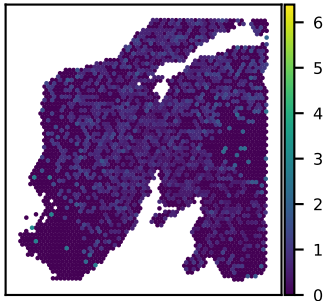
SNU24A DGLUCY expression Moran's I = 0.07
