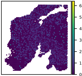
SNU24A RASSF8 expression Moran's I = 0.03
