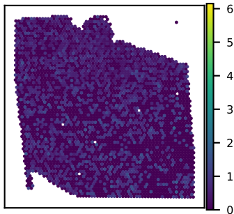
SNU27A SNAPIN expression Moran's I = 0.03
