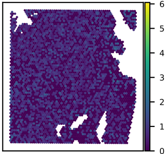
SNU51A HINT3 expression Moran's I = 0.01
