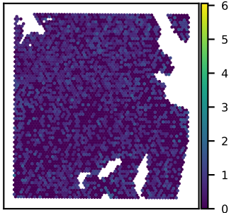
SNU51A TOM1 expression Moran's I = 0.02
