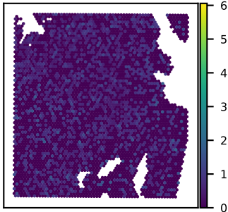
SNU51A CACHD1 expression Moran's I = 0.02
