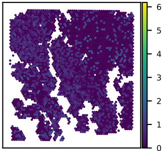
SNU16B TCEAL5 expression Moran's I = 0.05
