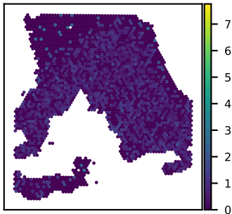
SNU18A CTTNBP2NL expression Moran's I = 0.06
