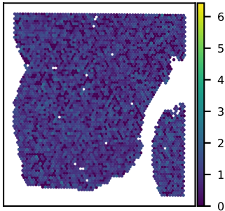
SNU25B GANAB expression Moran's I = 0.01
