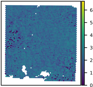
SNU43A SNRNP70 expression Moran's I = 0.07
