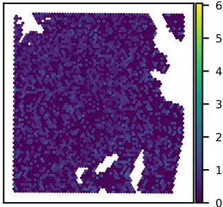
SNU51A RPAP2 expression Moran's I = 0.02
