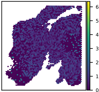
SNU24A PSMG1 expression Moran's I = 0.06
