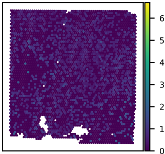
SNU43A C17orf97 expression Moran's I = 0.02
