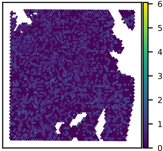
SNU51A ZDHHC16 expression Moran's I = 0.02
