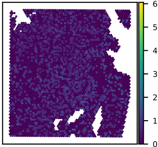
SNU51A SRRM1 expression Moran's I = 0.03
