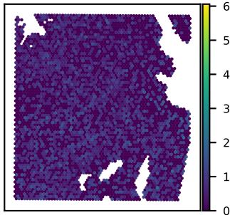
SNU51A ARMC6 expression Moran's I = 0.03
