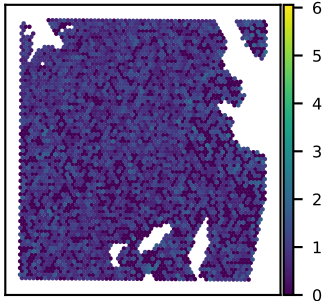
SNU51A SEC63 expression Moran's I = 0.01
