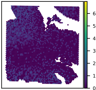
SNU24B UNC5A expression Moran's I = 0.23
