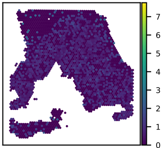
SNU18A FAM76B expression Moran's I = 0.04
