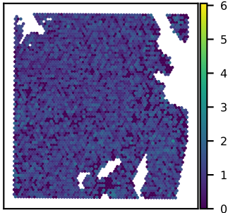
SNU51A LASP1 expression Moran's I = 0.04
