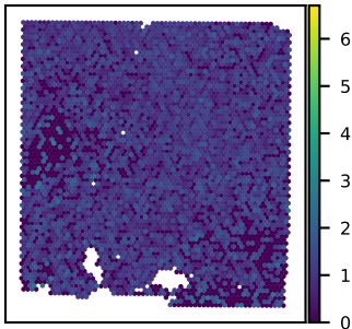
SNU43A FBXO7 expression Moran's I = 0.05
