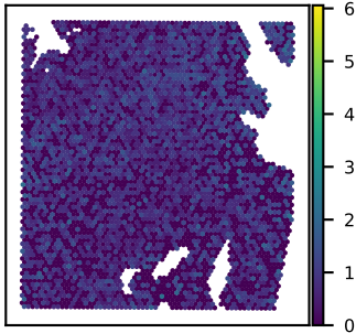
SNU51A CCNY expression Moran's I = 0.06
