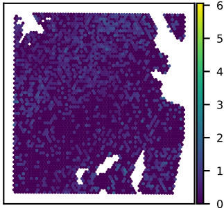
SNU51A LAIR1 expression Moran's I = 0.09
