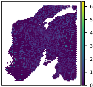
SNU24A GIMAP5 expression Moran's I = 0.04
