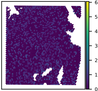
SNU51A PRPF39 expression Moran's I = 0.01
