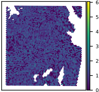
SNU51A DHX30 expression Moran's I = 0.03
