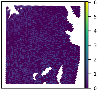
SNU51A CXADR expression Moran's I = 0.04
