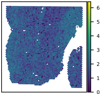
SNU25B PLEKHB1 expression Moran's I = 0.20
