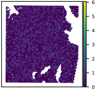
SNU51A CSNK1G3 expression Moran's I = 0.02
