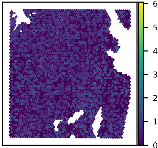
SNU51A ZZEF1 expression Moran's I = 0.01
