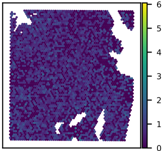
SNU51A NOC2L expression Moran's I = 0.03
