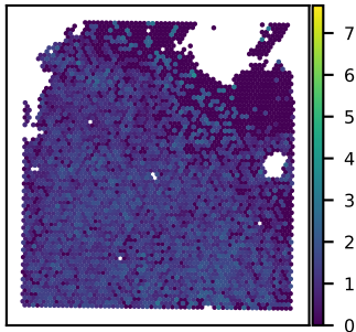
SNU21B HLA-DQA1 expression Moran's I = 0.29
