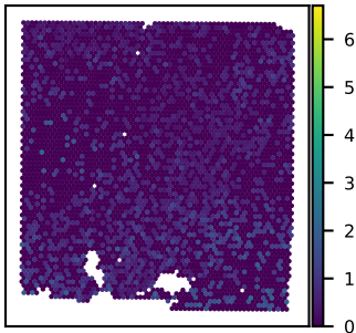
SNU43A CDKN2D expression Moran's I = 0.05
