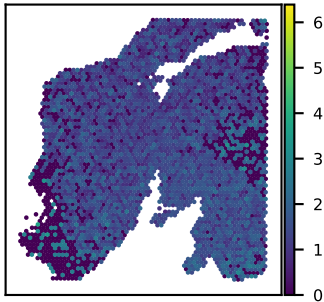
SNU24A PDGFRA expression Moran's I = 0.15
