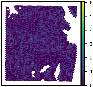
SNU51A BTBD6 expression Moran's I = 0.03
