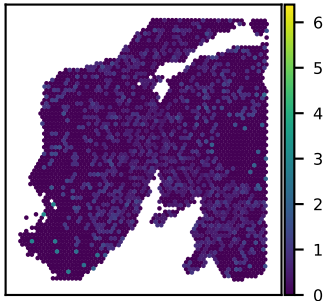
SNU24A NSDHL expression Moran's I = 0.03
